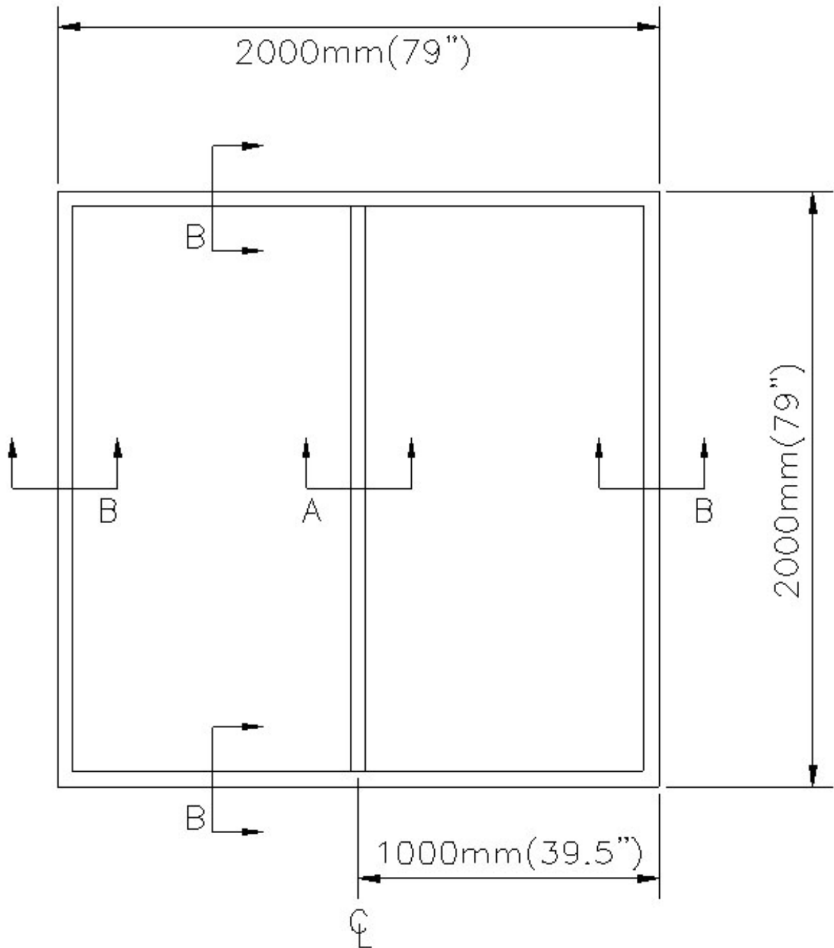
Figure 5-3 Nonresidential Windowwall Aluminum Frame Reference Product
