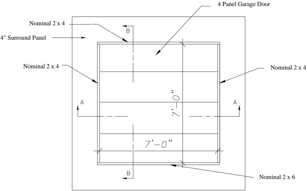
Figure A5-9 -- Garage Door Installation
