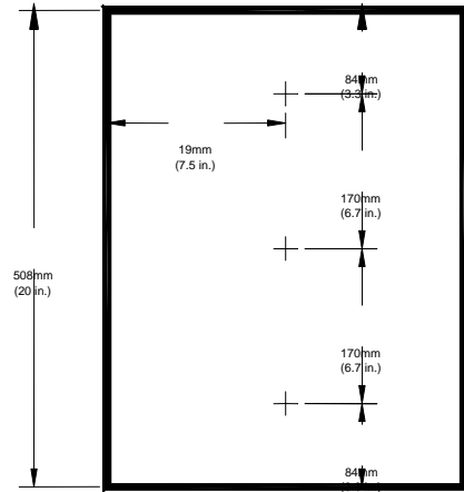
Figure A3.5 -- Attic Chamber Calibration Transfer Standard
