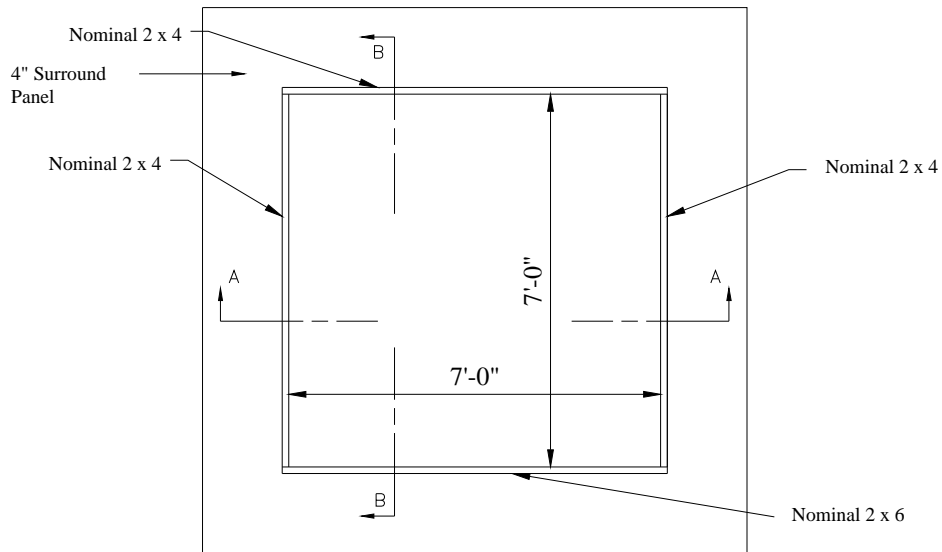
Figure A5-11 -- Rolling Door Installation
